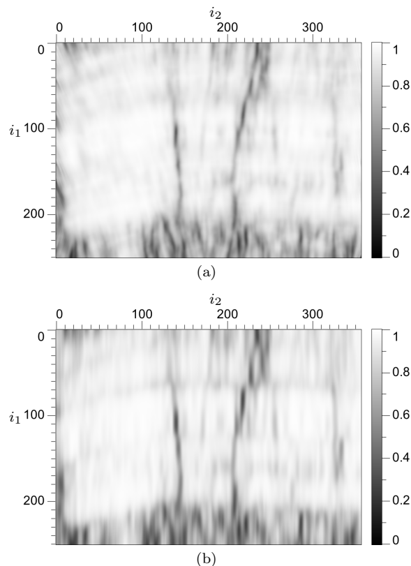
Figure 6. Structure-oriented semblance s_{v,w} (a) computed via structure-oriented smoothing and a more conventional slope-based semblance (b) for the image of Figure 2a.
