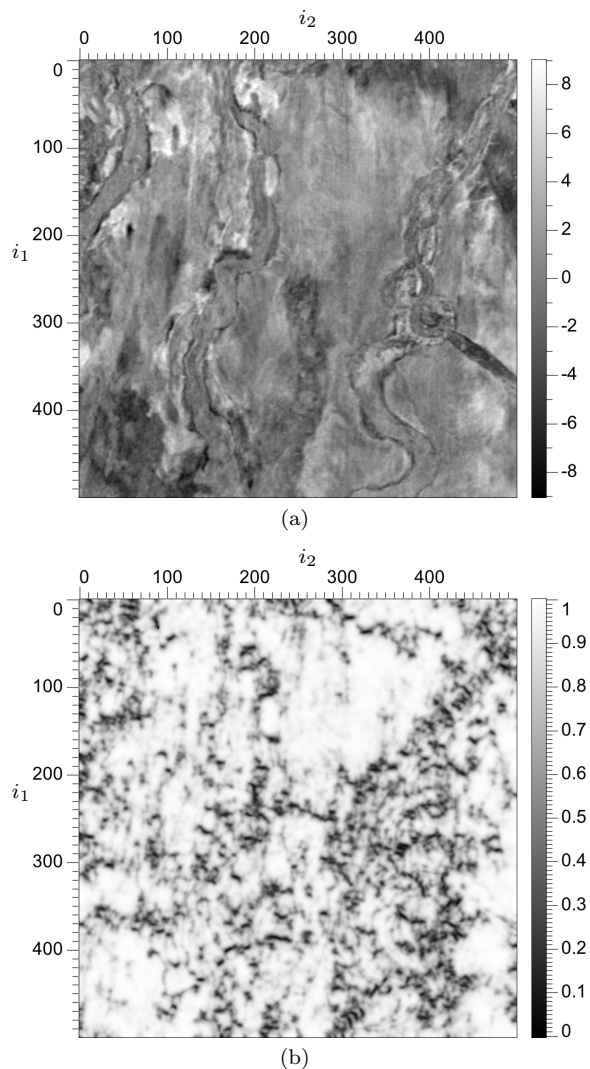
Figure 7. Features in a 2D horizontal slice (a) of a 3D image of channels have varying orientations. Structure-oriented semblance s_{v,u} (b) highlights amplitude variations along the linear trends of these features.
