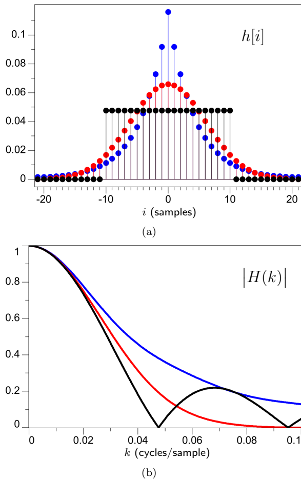
Figure 5. Three weighting sequences h[i] (a) and their Fourier amplitude spectra |H(k)| (b). Weights shown are boxcar (black), Gaussian (red), and smoothed exponential (blue).
