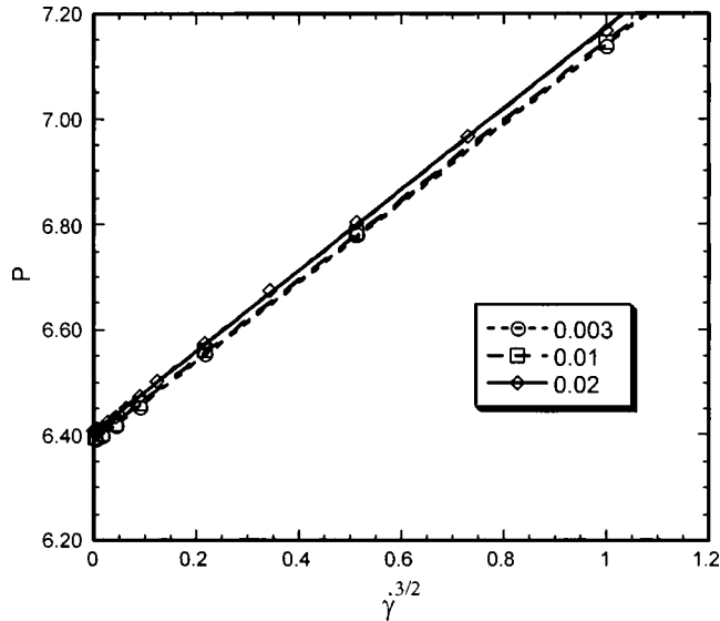
FIG. 5. Energy simulations for 2048 particles using different time-step sizes. The open circles are from simulations of step size 0.003, open squares from step size 0.01, and open diamonds from step size 0.02. The lines are linear fit curves of the data points with respect to \gamma^{3/2} . The error bars are too small to be displayed.
