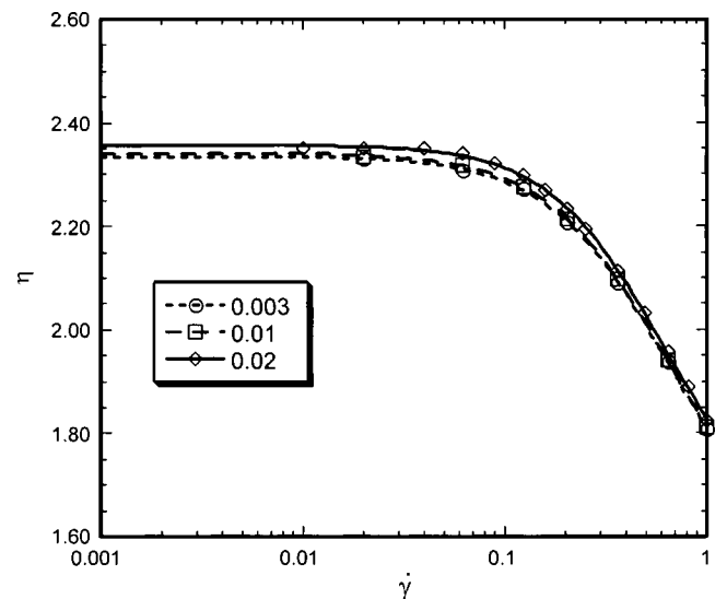
FIG. 7. The shear viscosities of WCA fluid of 2048 particles measured using different time-step sizes as a function of shear rate \gamma . The open circle, square, and diamond symbols correspond to time step sizes 0.003, 0.01, and 0.02. The lines are fitted Cross model curves.
