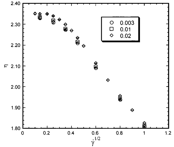
FIG. 6. Simulated shear viscosities as a function of \gamma^{1/2} in a 2048 particle system using the proposed algorithm with different time-step sizes 0.003, 0.01, and 0.02. The error bars are shown in the figures, which are small.
