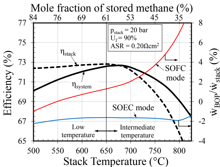
Figure 8.5: Roundtrip stack and system efficiency (left), net BOP power produced ( \dot{W}_{BOP} ) relative to stack power ( \dot{W}_{stack} ) (right), and stored methane mole fraction (top) vs. stack temperature.
