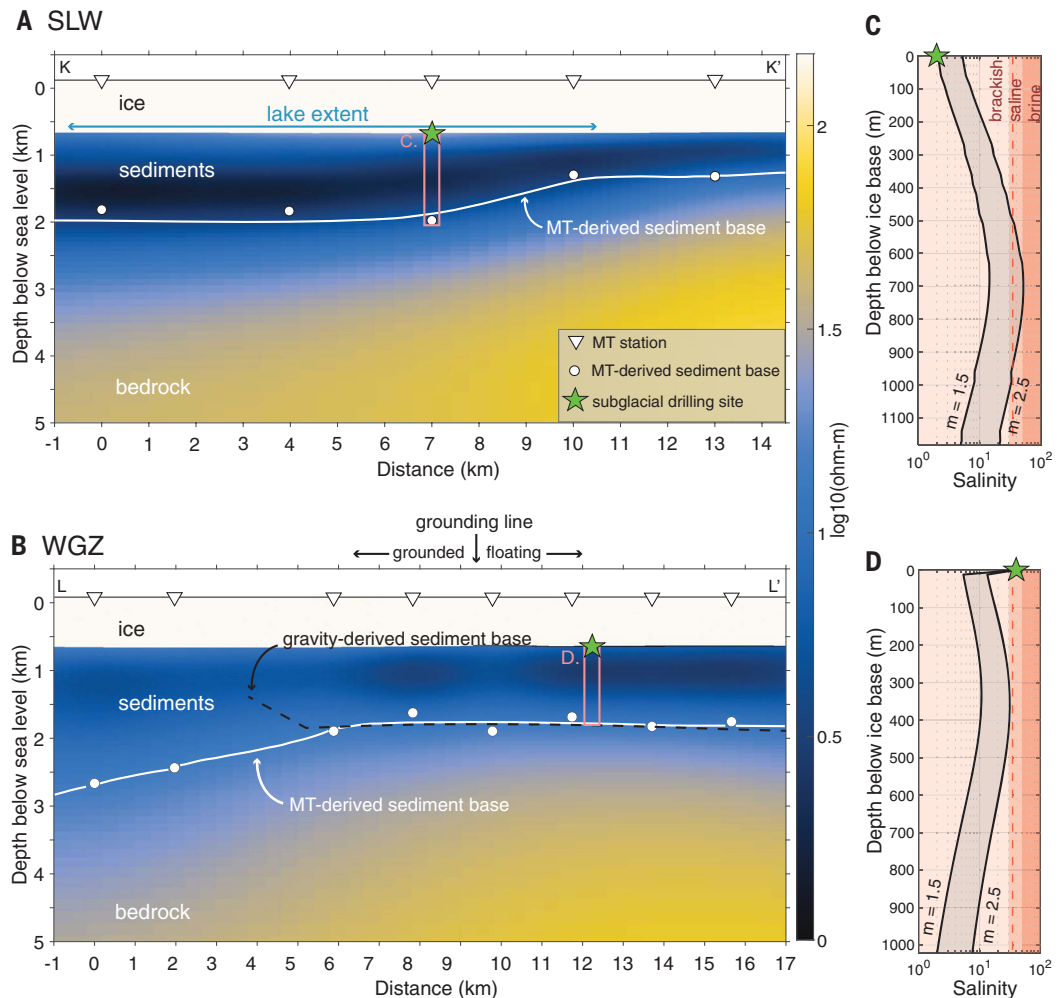
Fig. 2. Resistivity models and inferred groundwater salinity.
